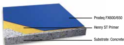
Water Containment System
