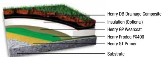
Plaza Deck System
