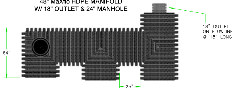
24" ACCESS RISER @ 3' TALL
