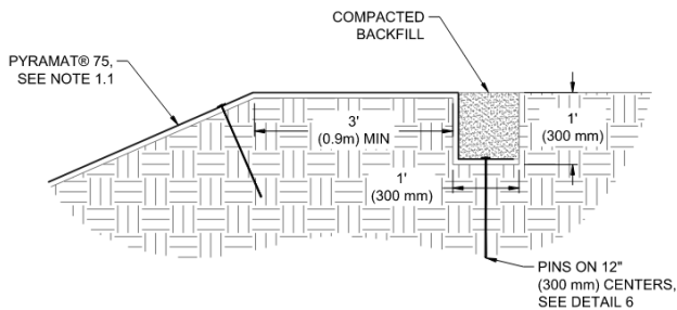
Figure 1: Crest of Slope (COS) trench
