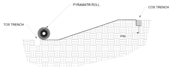
Figure 6: Placement of PROPER Pyramat across slope
