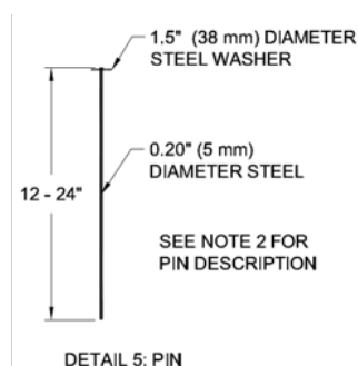
Figure 6: Securing pin
