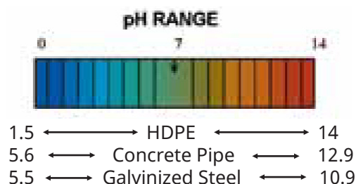
Corrosion Resistance
