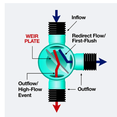
Weir Structure
