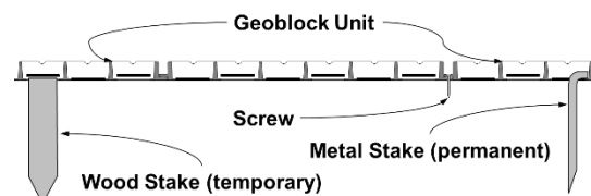
Figure 9 Anchoring Possibilities
