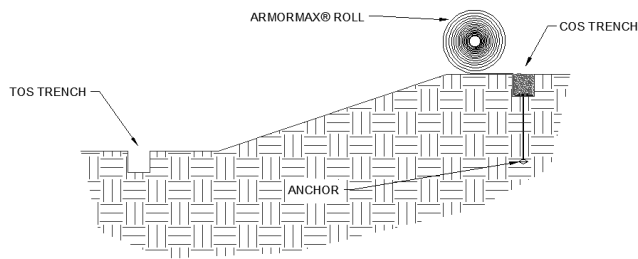
Figure 5: Crest of Slope (COS) Trench Placement
