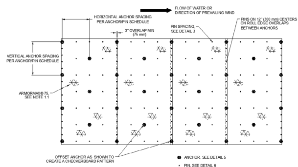
Figure 8: Example of Anchor Pattern - 0.5 Anchors/yd 2
