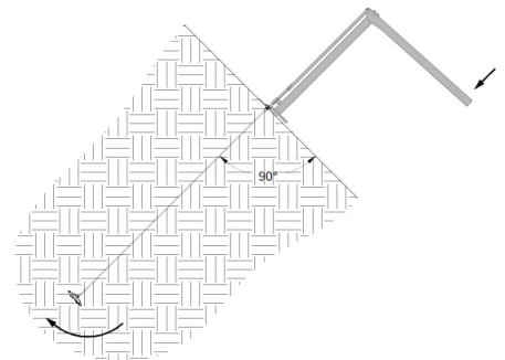
Figure 20: Use JackJaw Setting Tool to Set Anchor
