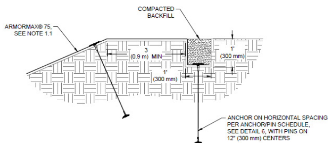
Figure 1A: Crest of Slope (COS) Trench
