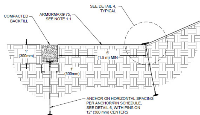
Figure 2: Toe of Slope (TOS) Trench
