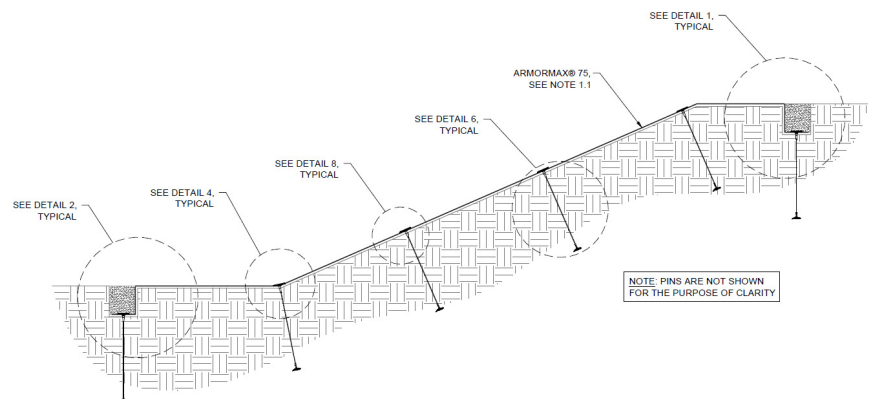
Figure 13: Completed Slope Isometric View
